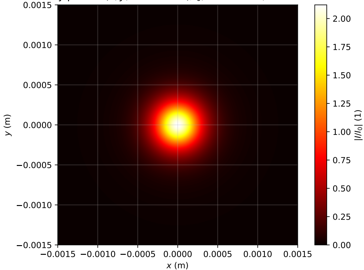
Intensity profile I(x, y, z = 1.990\text{m})/I_0 , \text{Pin}=1.0\text{Pcr} , artificial time
